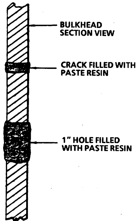
FIGURE 8-12. Bulkhead Repair.
