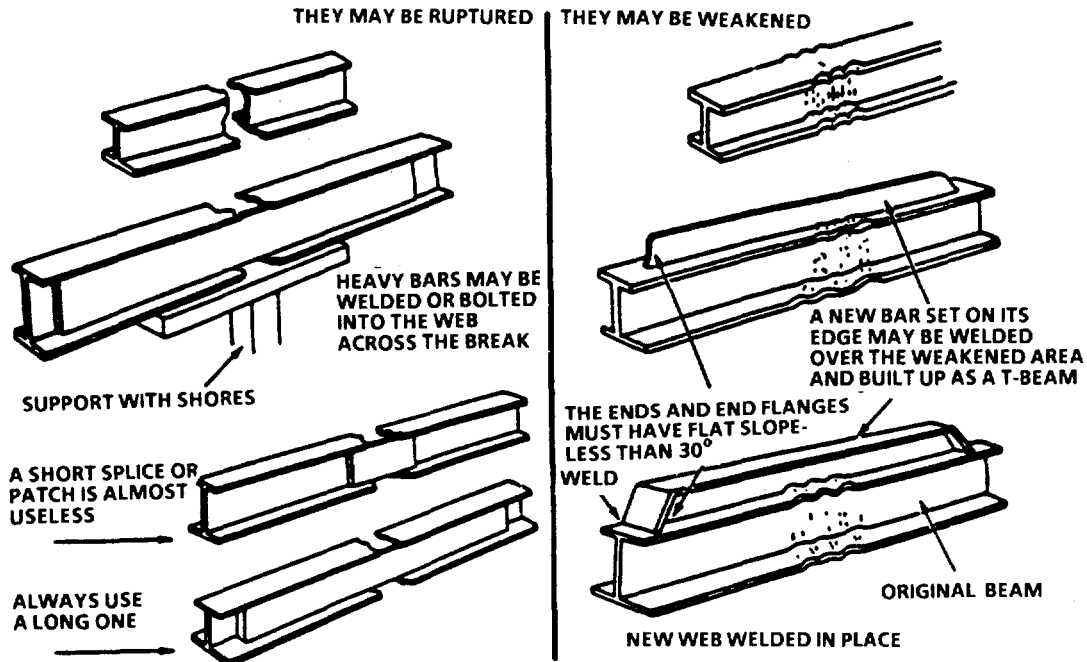
FIGURE 8-3. Strengthening Beams and Frames.
