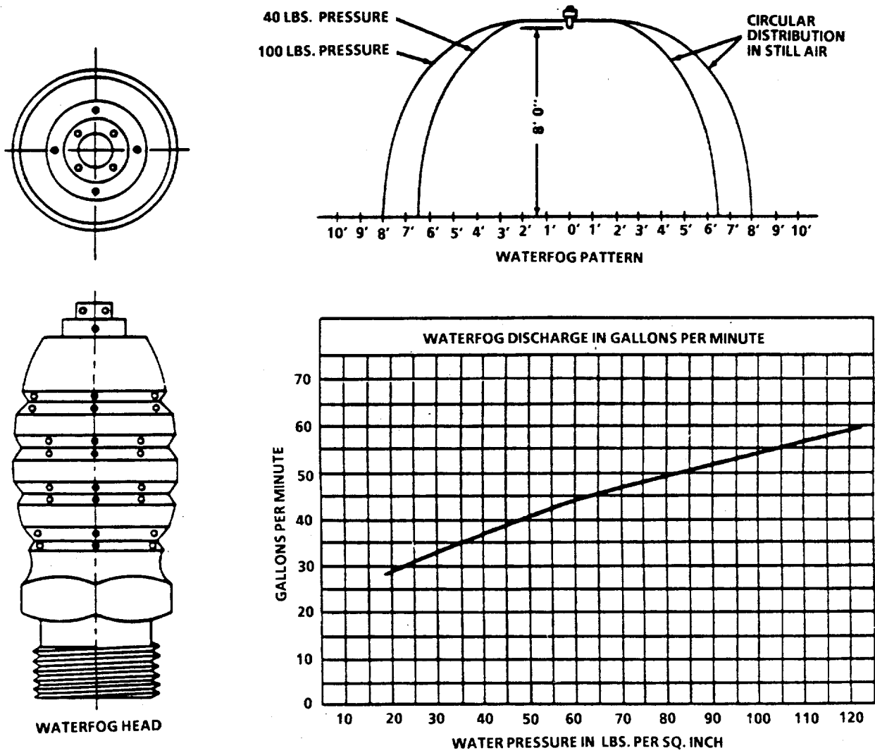
FIGURE 6-3. Low-Velocity Fog Pattern.
