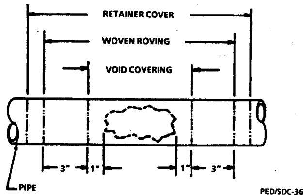
FIGURE 8-9. Sequence of Applied Patch Materials.
