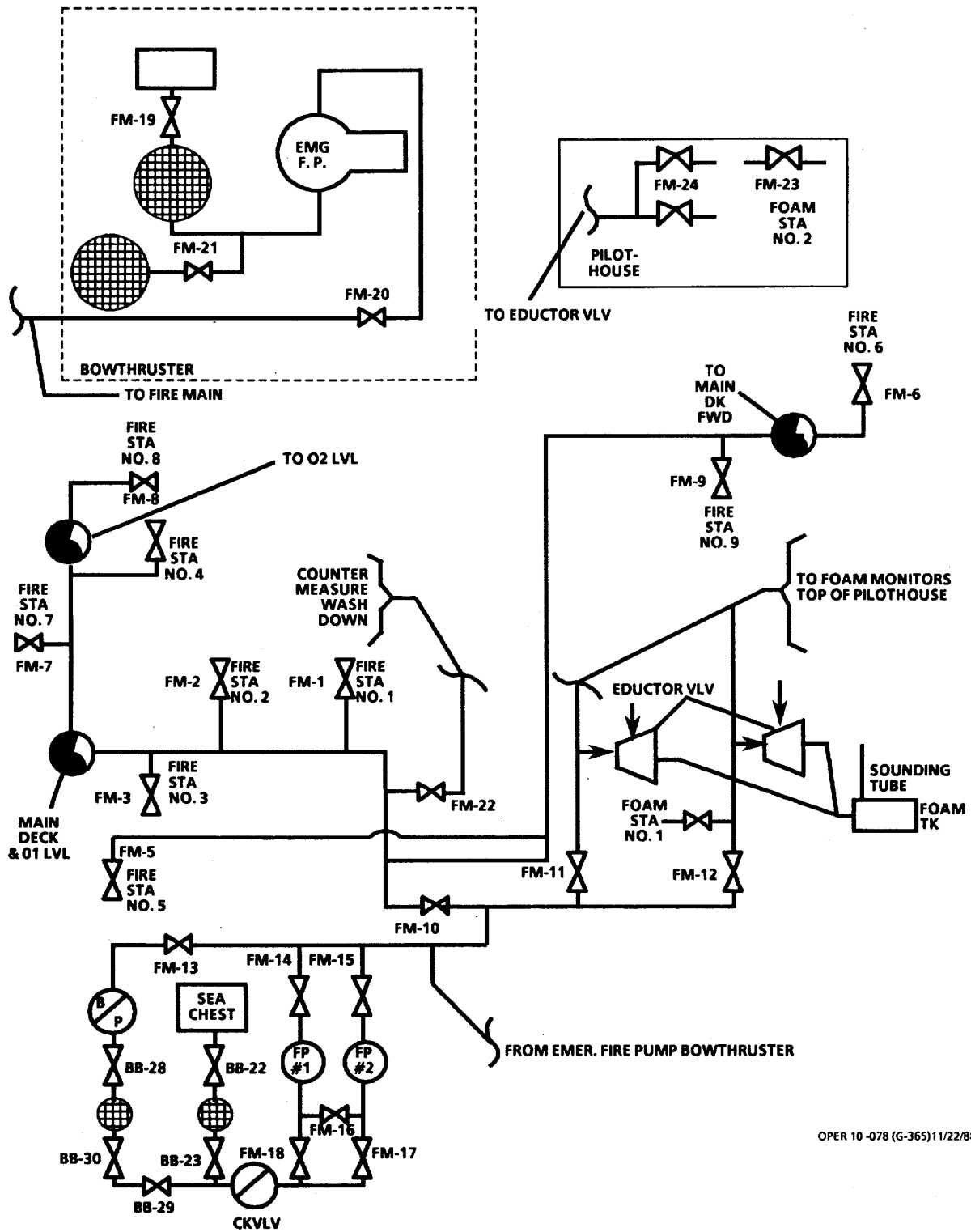
FIGURE 6-5. Fire Main System.
