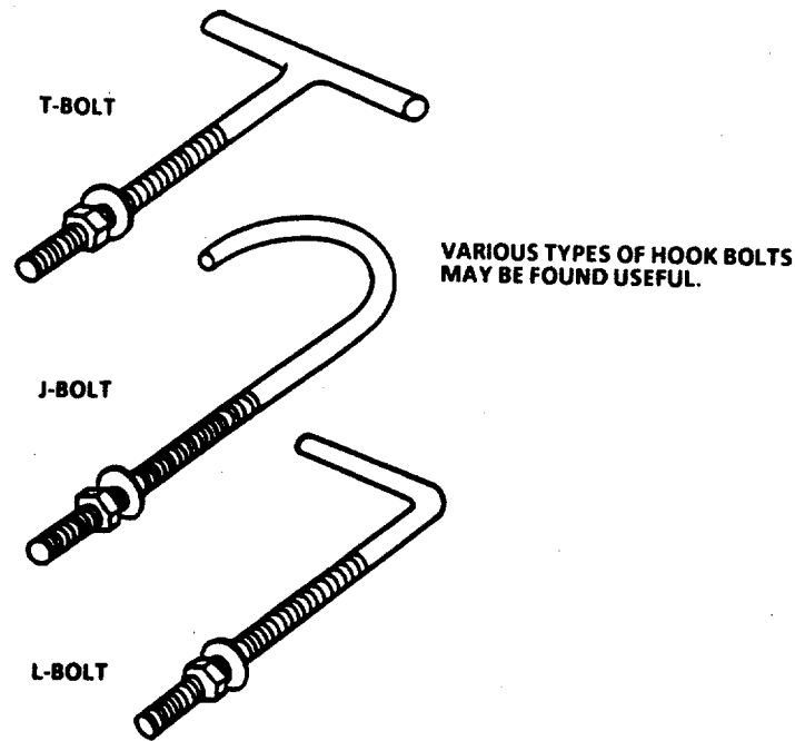
FIGURE 8-1. Types of Hook Bolts
