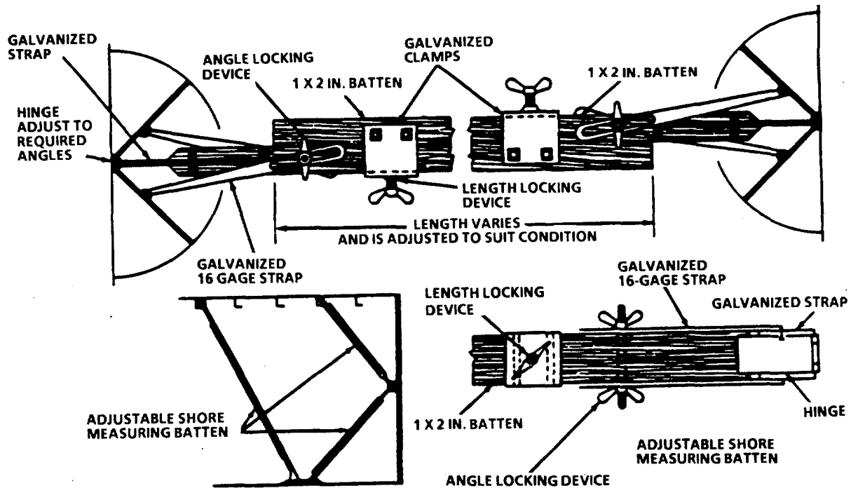
FIGURE 7-1. Adjustable Shoring Batten.
