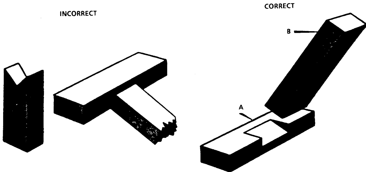
FIGURE 7-5. Notching a Shore to Fit Another.
