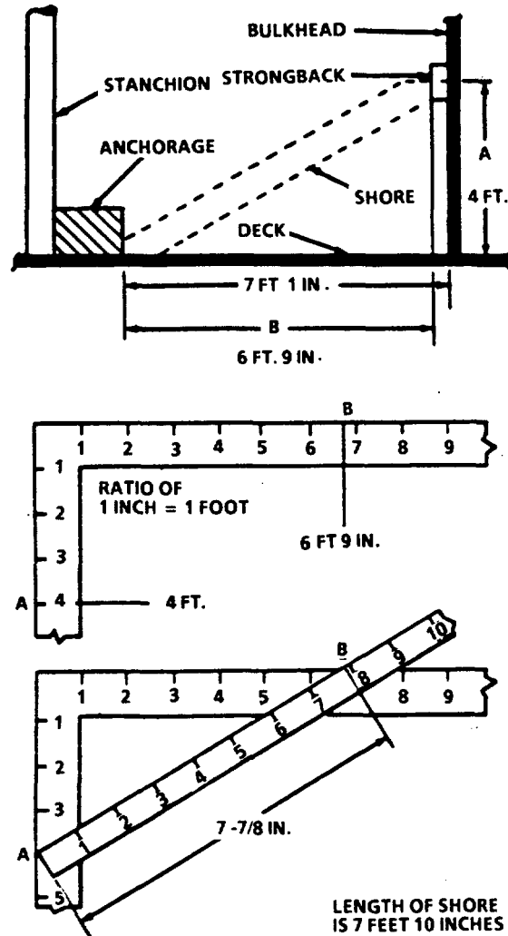
FIGURE 7-2. Determining Length of Shore.
