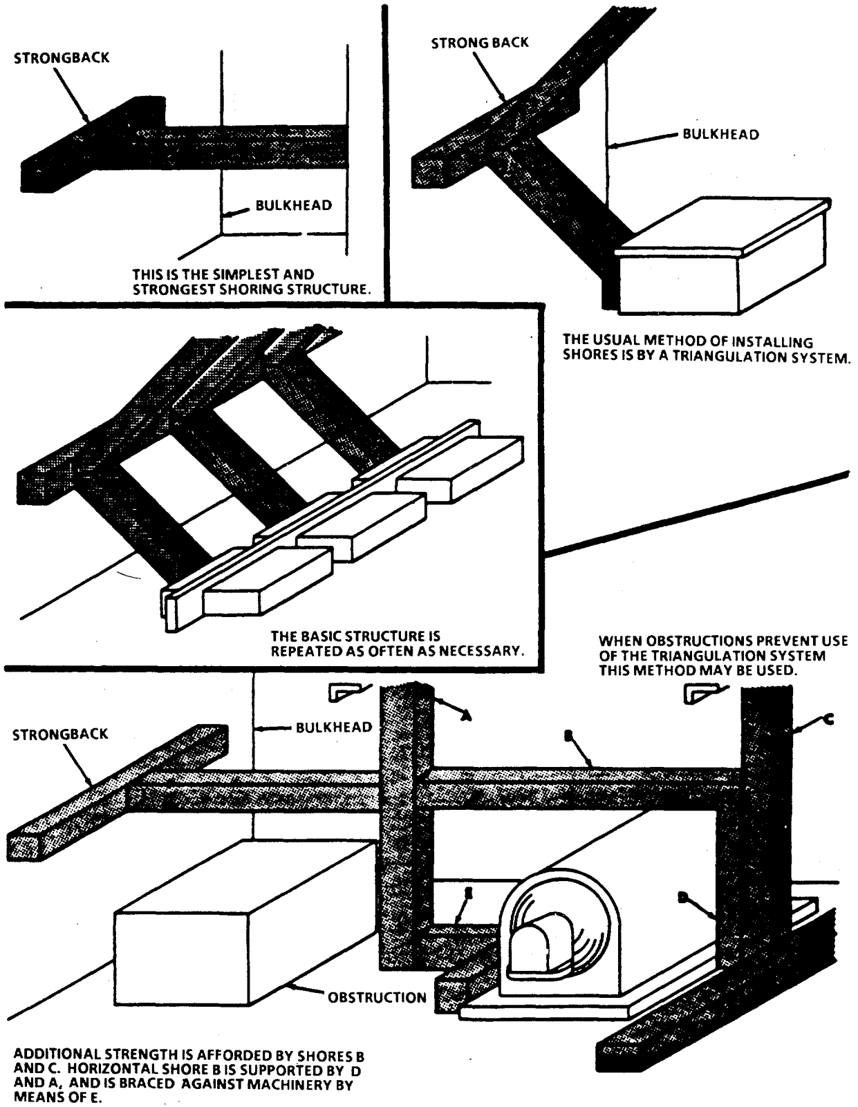
FIGURE 7-6. Shoring Against Horizontal Pressure.
