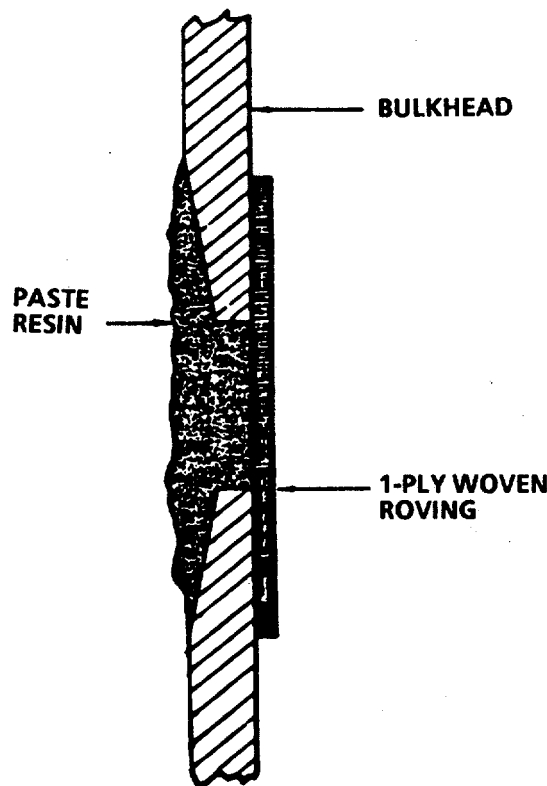
FIGURE 8-13. Combination Patch Repairs to Metal or Wooden Bulkheads.
